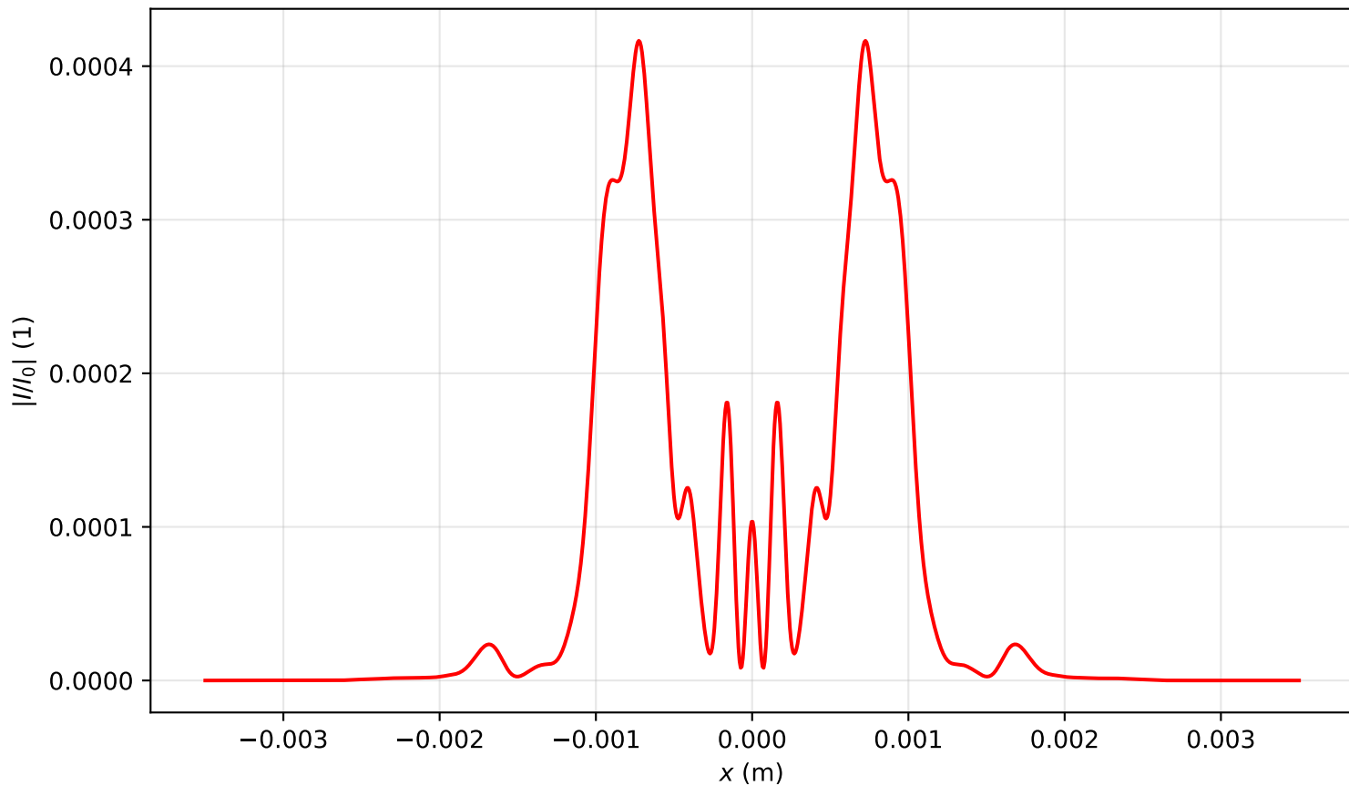
Intensity profile I(x, y = 0, z = 0.716)/I_0 , P_{in}=15.0\text{Pcr} , artificial time
