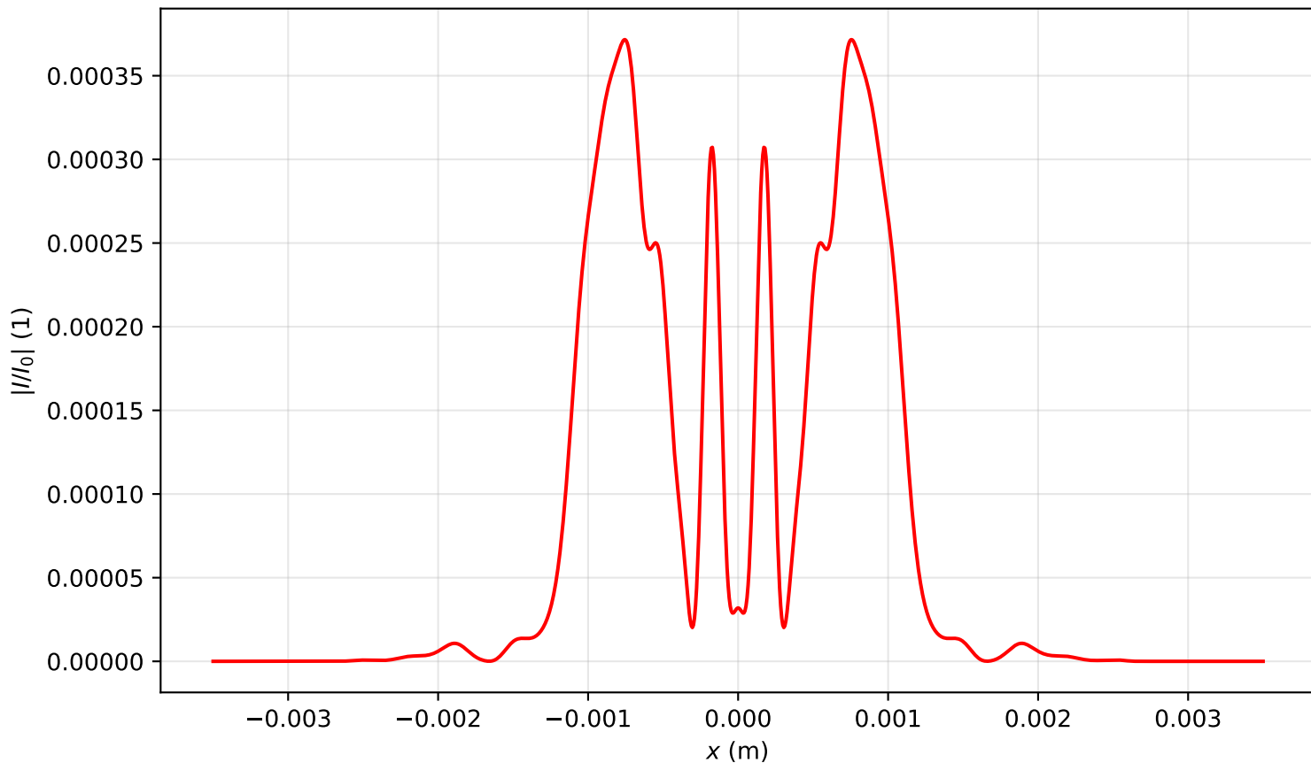
Intensity profile I(x, y = 0, z = 0.796)/I_0 , P_{in}=15.0P_{cr} , artificial time
