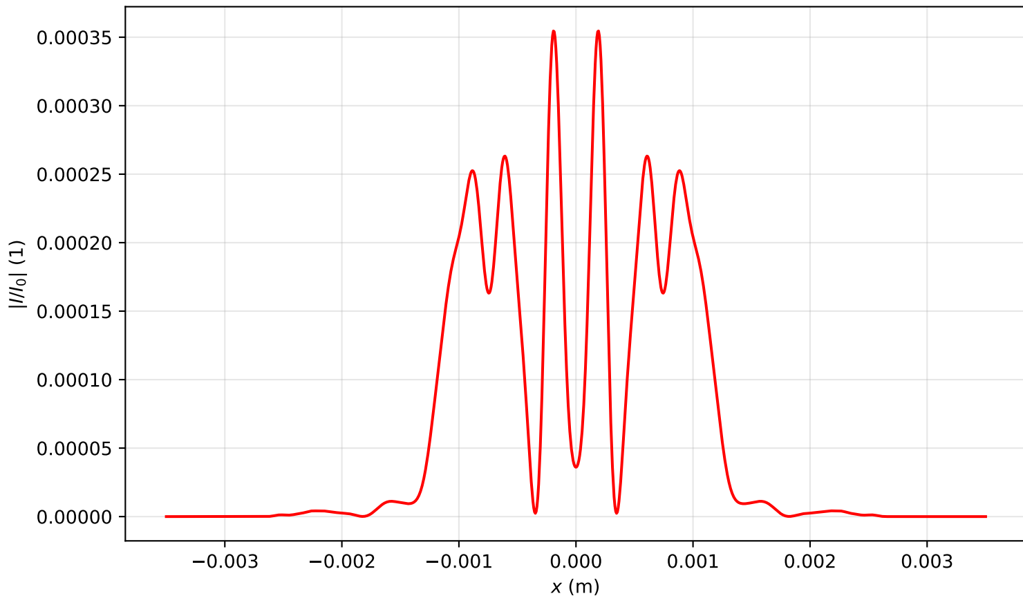
Intensity profile I(x, y = 0, z = 0.876)/I_0 , P_{in}=15.0\text{Pcr} , artificial time
