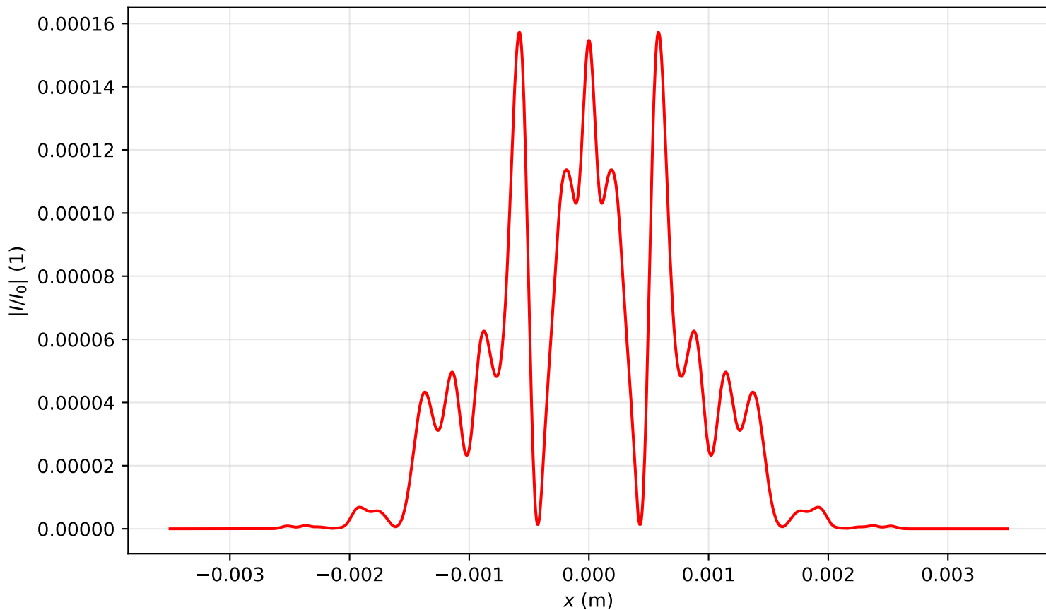
Intensity profile I(x, y = 0, z = 1.035)/I_0 , P_{in}=15.0P_{cr} , artificial time
