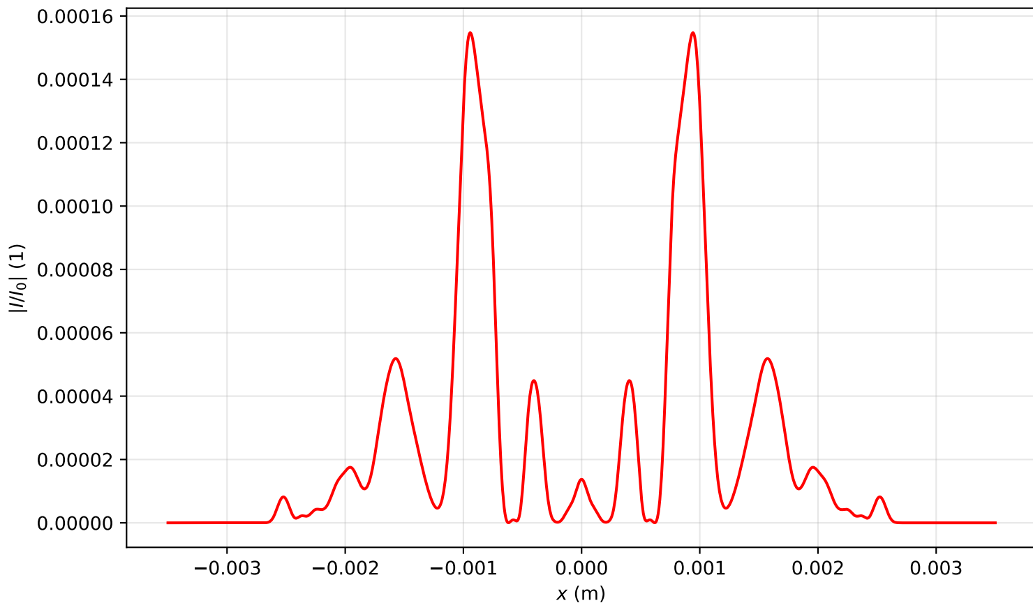
Intensity profile I(x, y = 0, z = 1.592)/I_0 , P_{in}=15.0P_{cr} , artificial time
