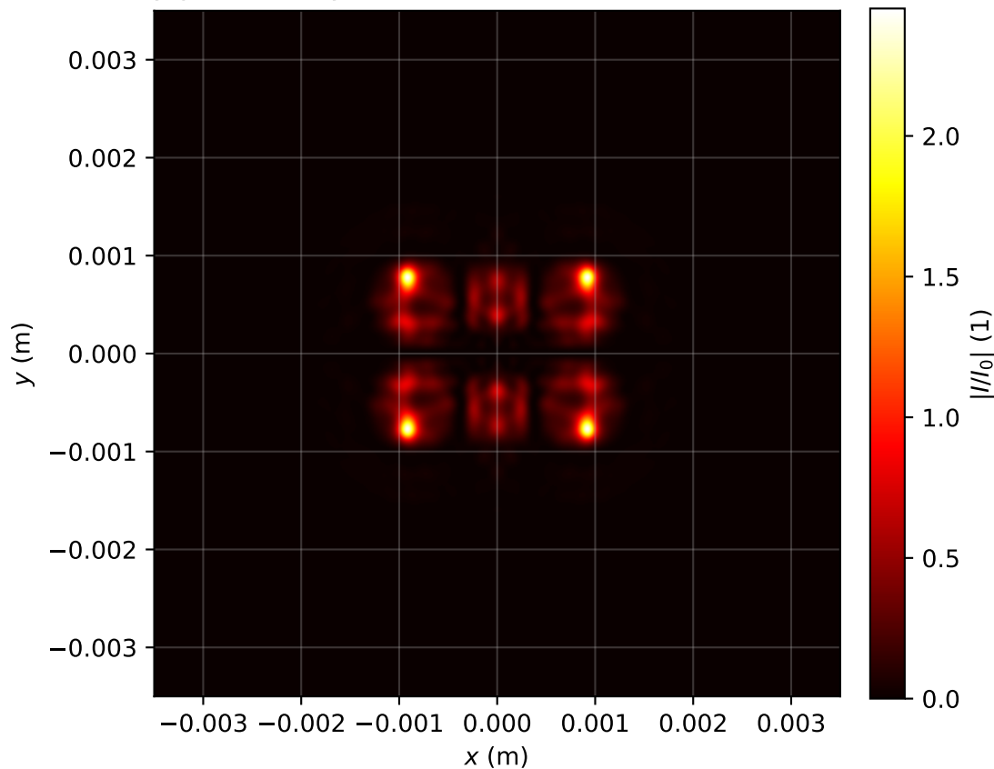
Intensity profile I(x, y, z = 0.716)/I_0 , P_{in}=15.0P_{cr} , artificial time
