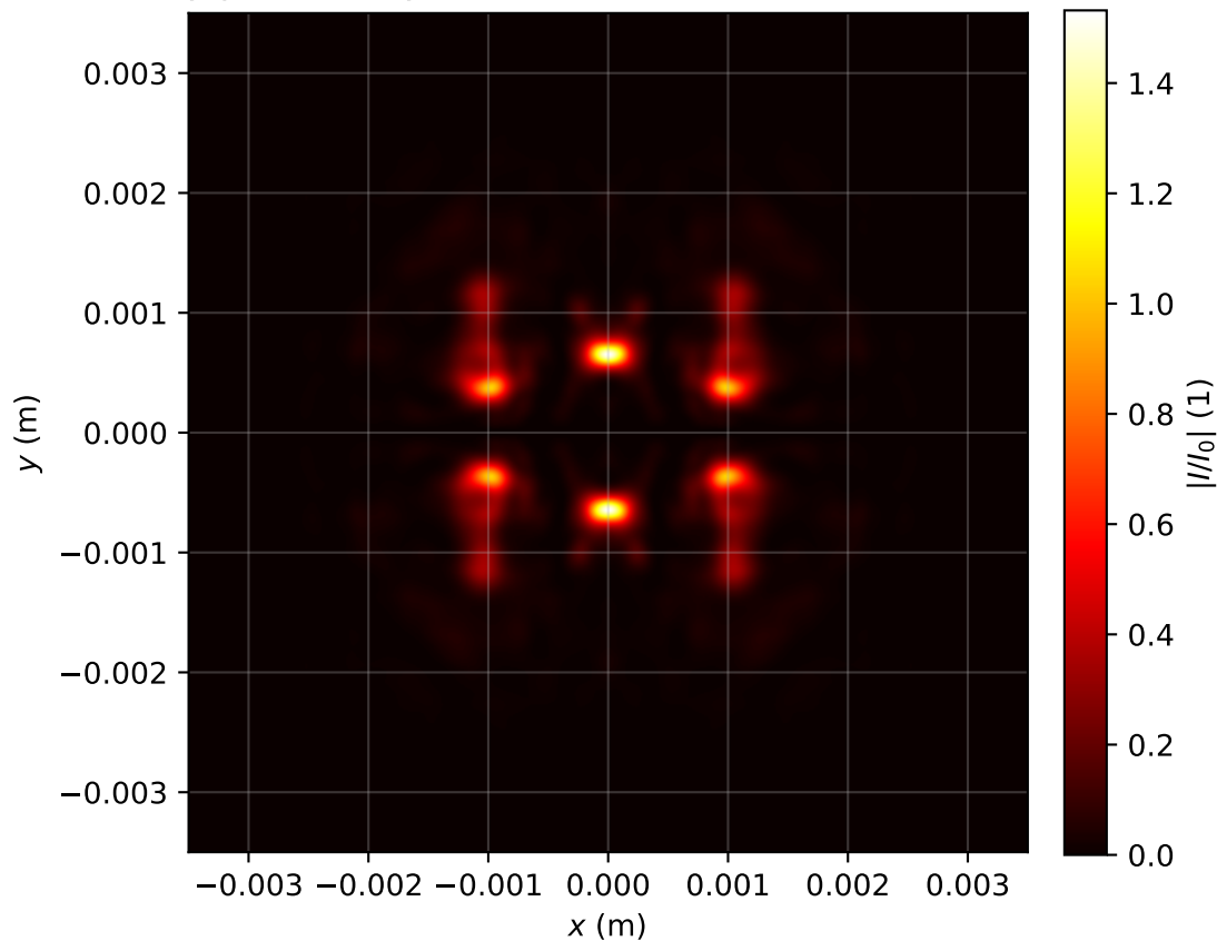
Intensity profile I(x, y, z = 1.592)/I_0 , P_{in}=15.0P_{cr} , artificial time
