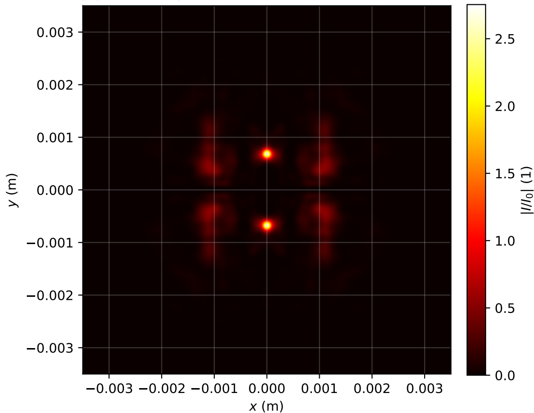
Intensity profile I(x, y, z = 1.672)/I_0 , P_{in}=15.0\text{Pcr} , artificial time
