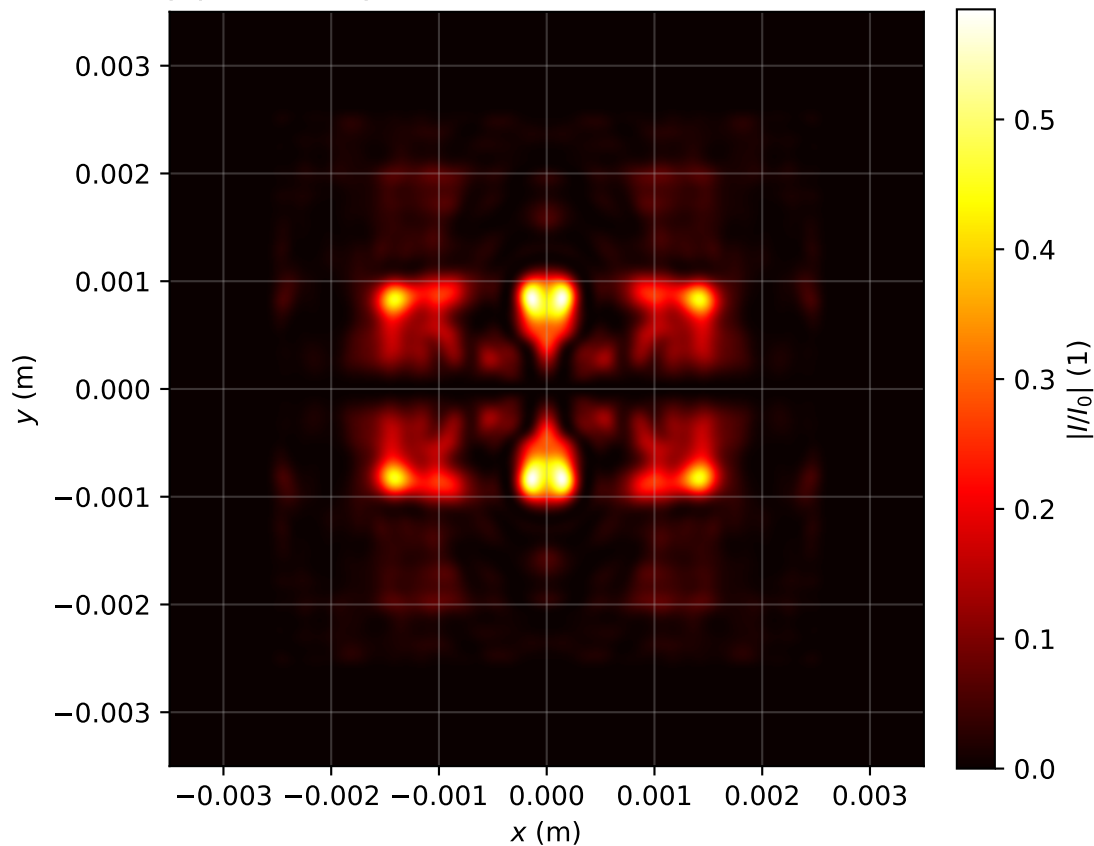
Intensity profile I(x, y, z = 2.149)/I_0 , P_{in}=15.0P_{cr} , artificial time
