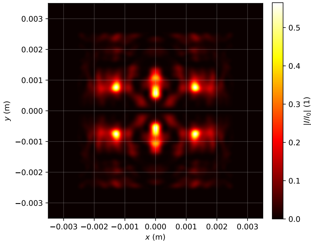
Intensity profile I(x, y, z = 2.548)/I_0 , P_{in}=15.0\text{Pcr} , artificial time
