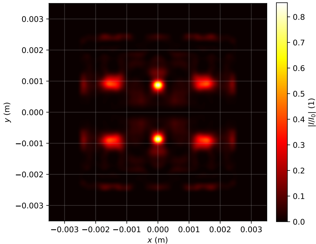
Intensity profile I(x, y, z = 3.025)/I_0 , P_{in}=15.0P_{cr} , artificial time
