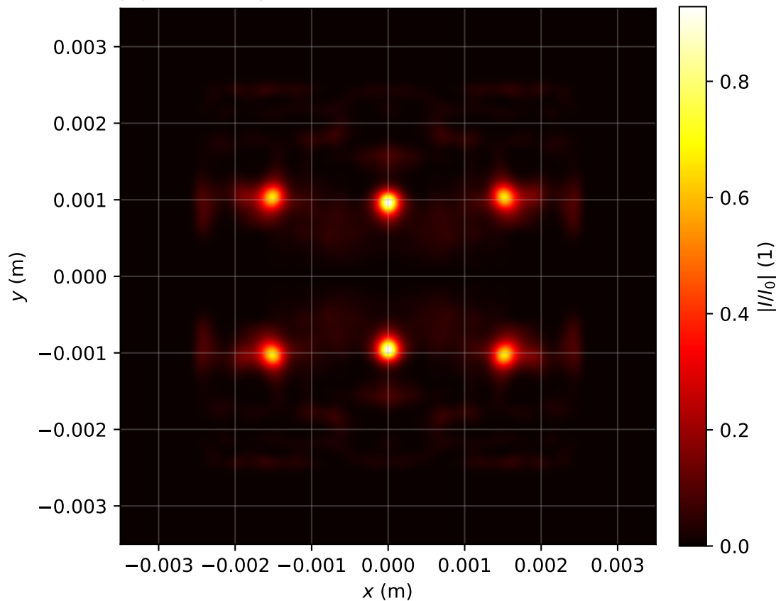
Intensity profile I(x, y, z = 3.264)/I_0 , P_{in}=15.0\text{Pcr} , artificial time
