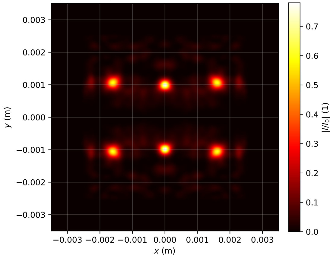
Intensity profile I(x, y, z = 3.423)/I_0 , P_{in}=15.0P_{cr} , artificial time
