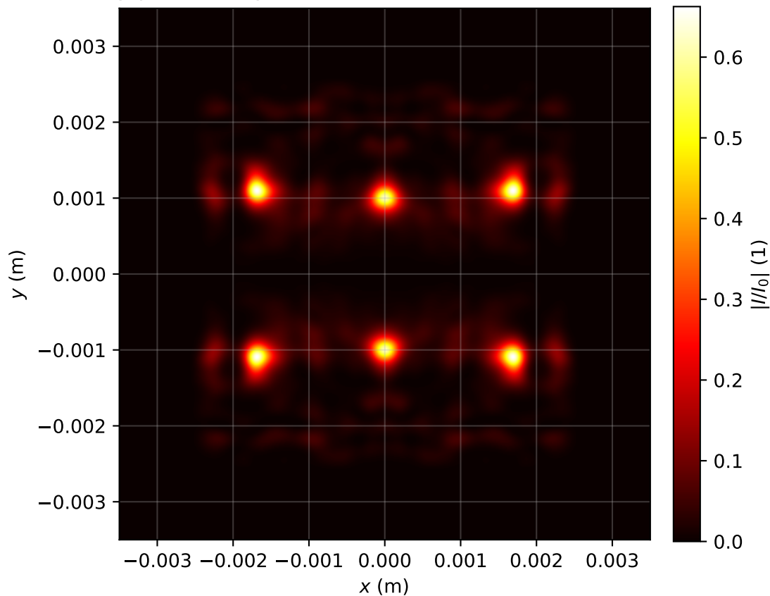
Intensity profile I(x, y, z = 3.582)/I_0 , P_{in}=15.0P_{cr} , artificial time
