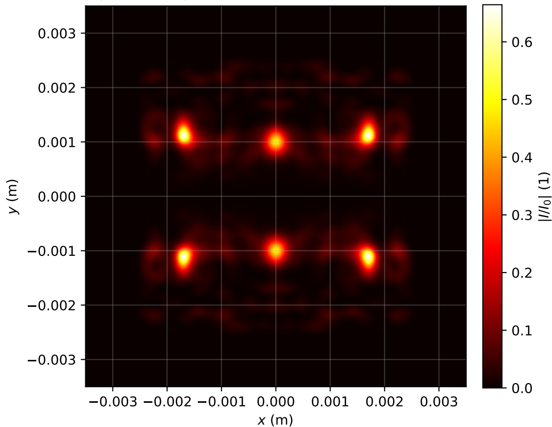
Intensity profile I(x, y, z = 3.662)/I_0 , P_{in}=15.0P_{cr} , artificial time
