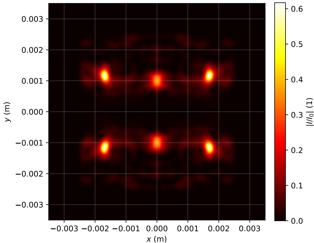
Intensity profile I(x, y, z = 3.742)/I_0 , P_{in}=15.0P_{cr} , artificial time
