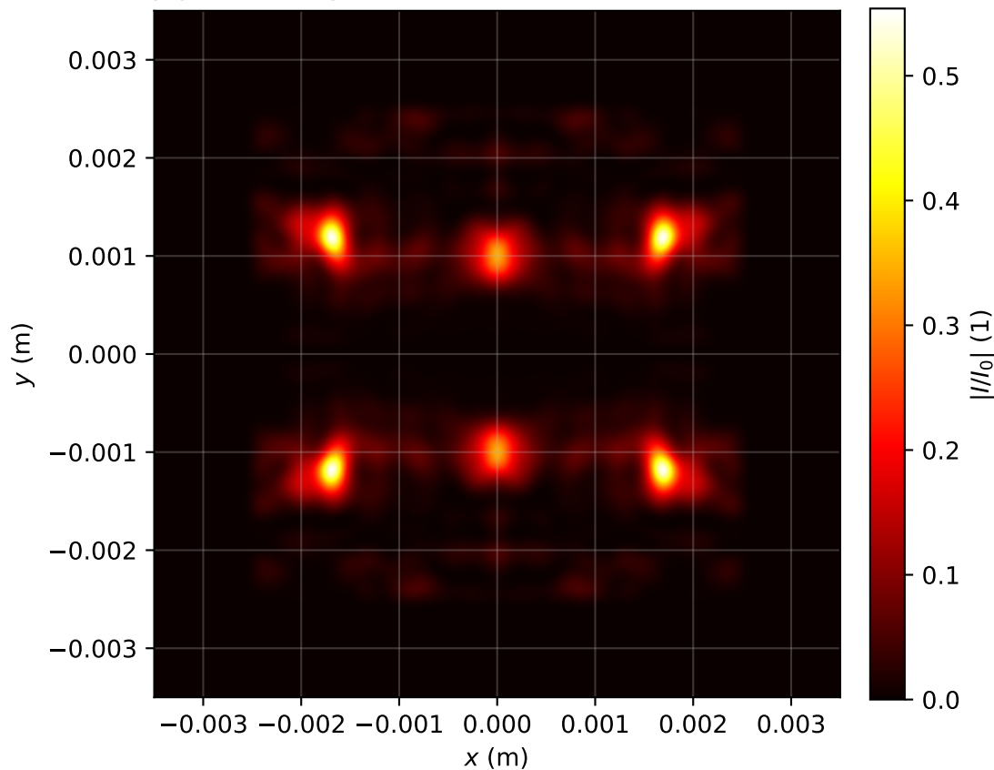
Intensity profile I(x, y, z = 3.821)/I_0 , P_{in}=15.0P_{cr} , artificial time
