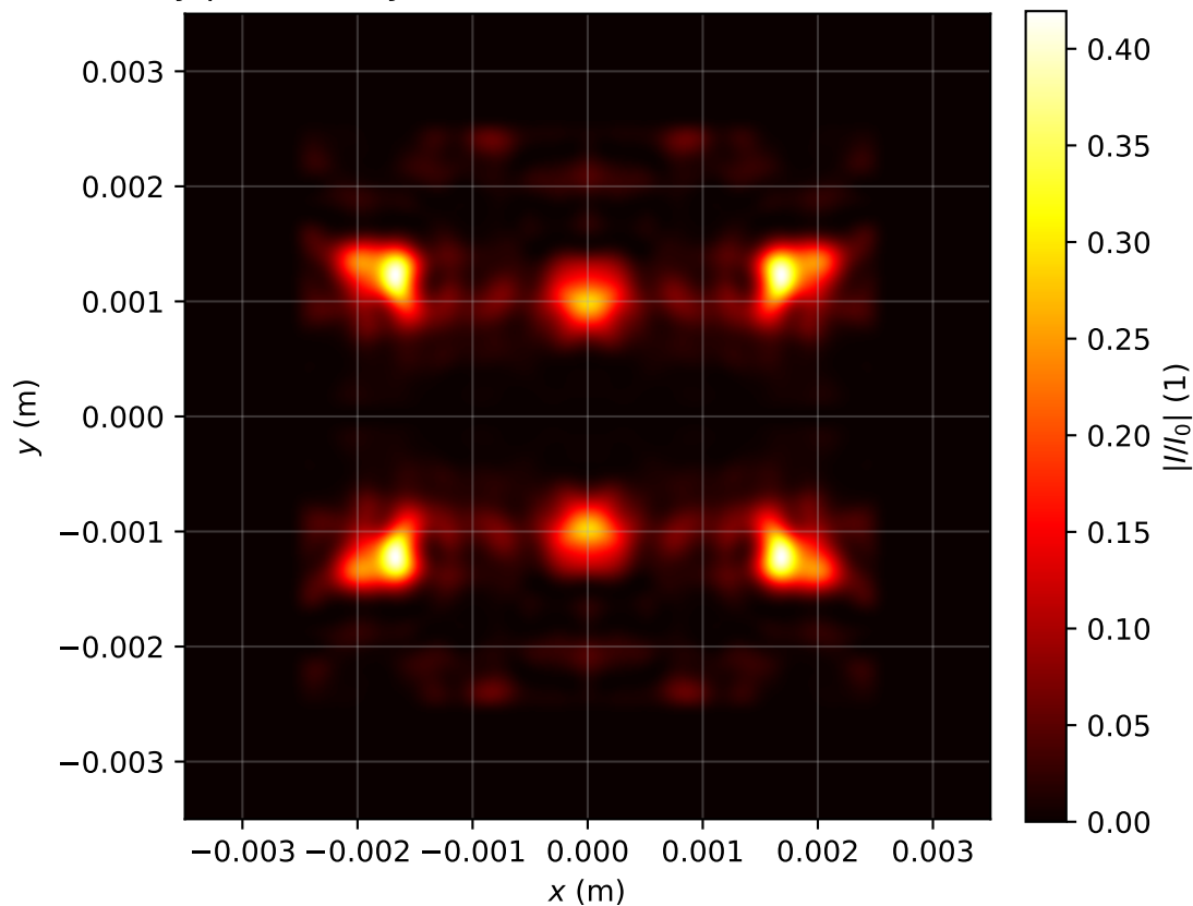
Intensity profile I(x, y, z = 3.901)/I_0 , P_{in}=15.0P_{cr} , artificial time
