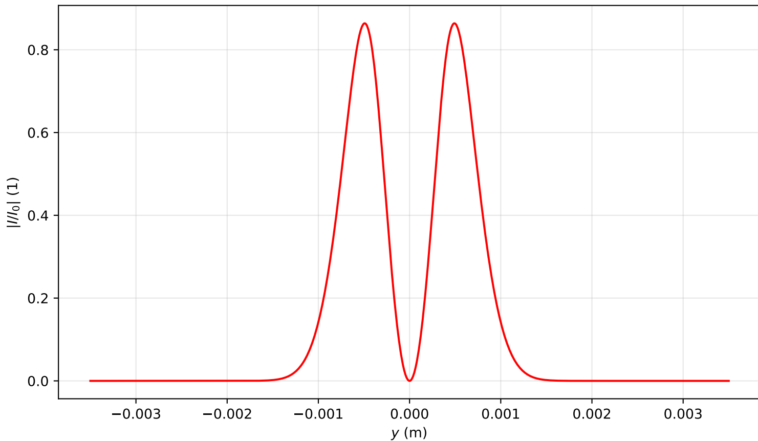
Intensity profile I(x=0, y, z=0.080)/I_0 , P_{in}=15.0P_{cr} , artificial time
