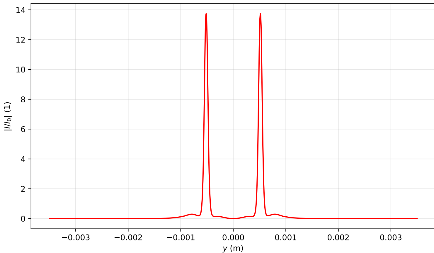
Intensity profile I(x=0, y, z=0.398)/I_0 , \text{Pin}=15.0\text{Pcr} , artificial time
