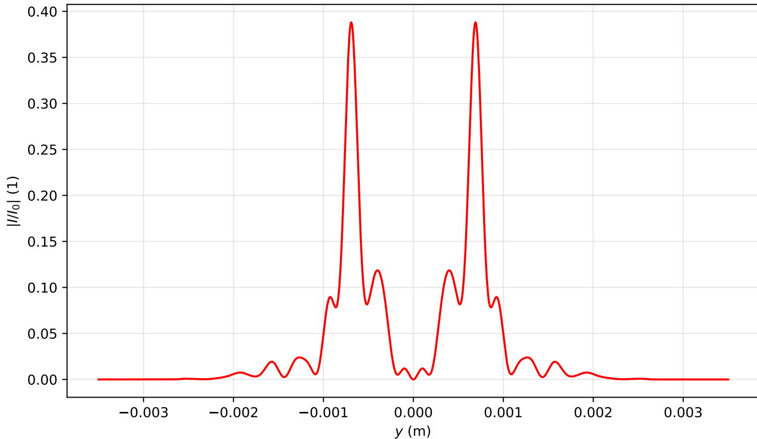
Intensity profile I(x=0, y, z=0.876)/I_0 , P_{in}=15.0P_{cr} , artificial time
