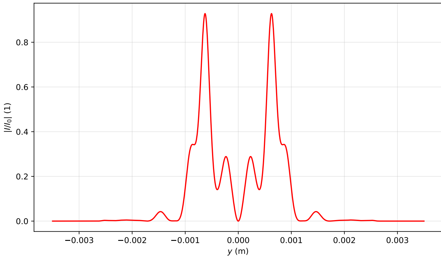
Intensity profile I(x=0, y, z=1.035)/I_0 , P_{in}=15.0P_{cr} , artificial time
