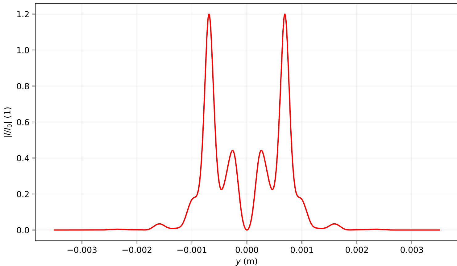
Intensity profile I(x=0, y, z=1.115)/I_0 , P_{in}=15.0P_{cr} , artificial time
