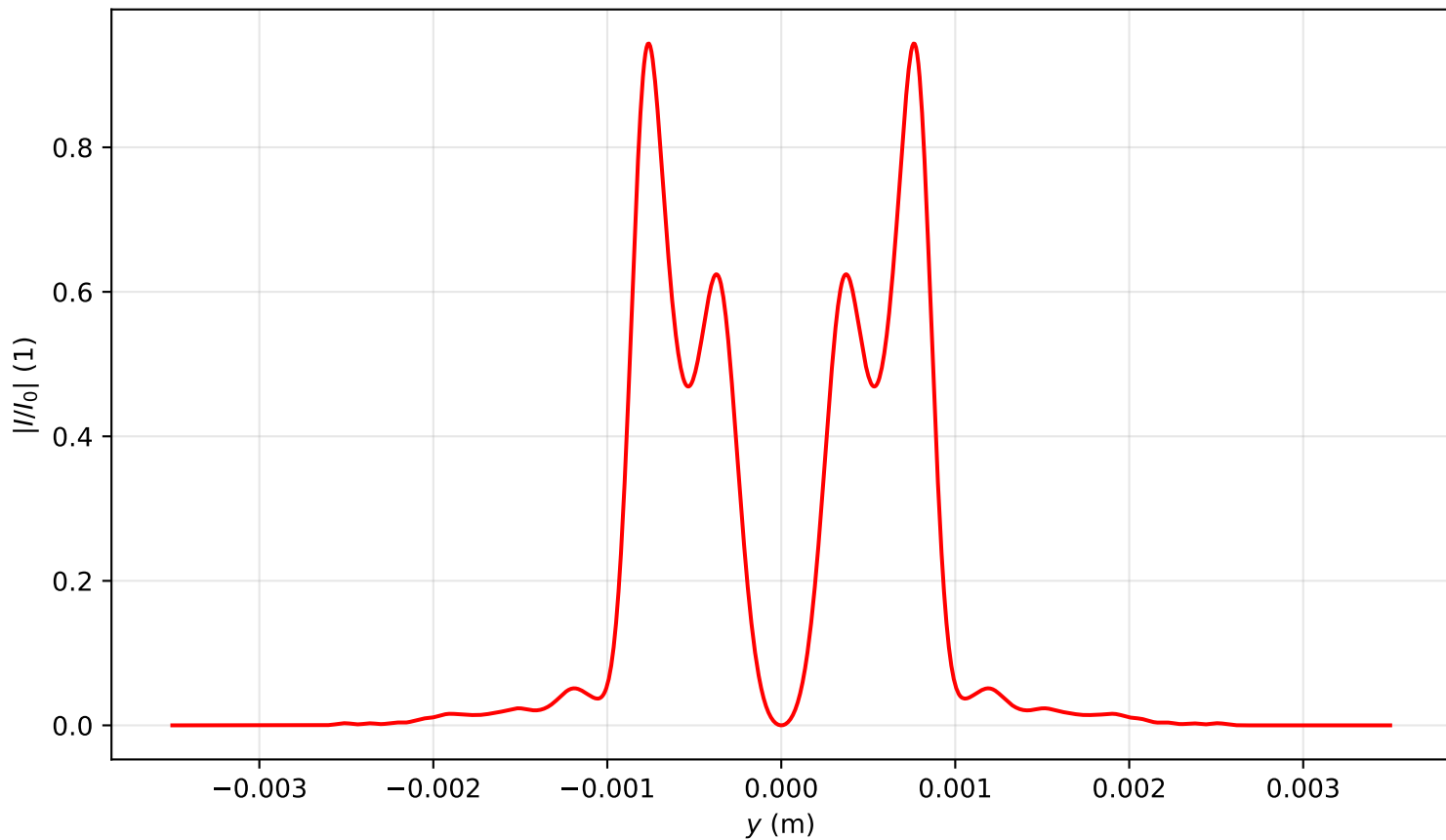
Intensity profile I(x=0, y, z=1.274)/I_0 , Pin=15.0Pcr, artificial time
