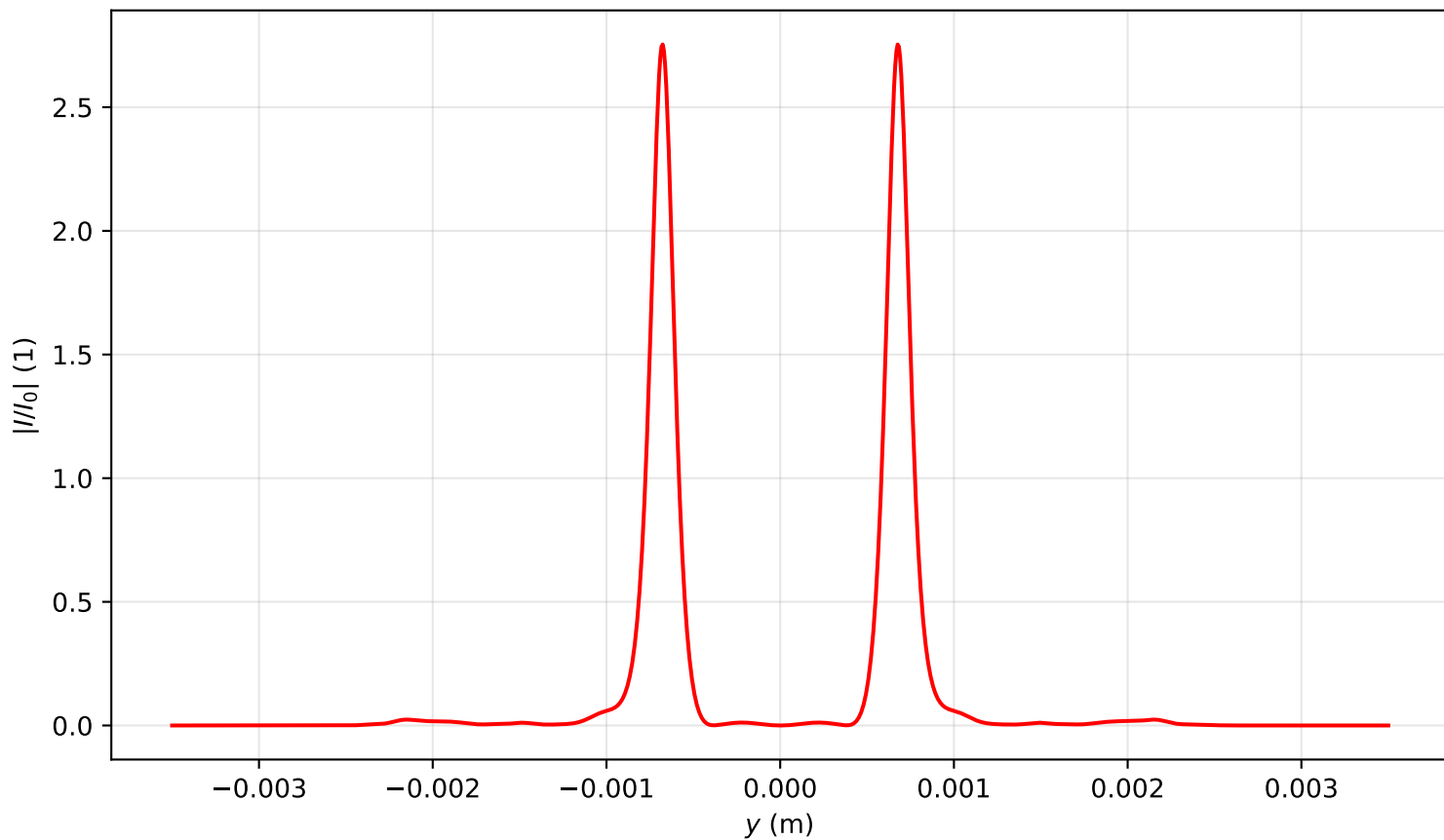
Intensity profile I(x=0, y, z=1.672)/I_0 , P_{in}=15.0P_{cr} , artificial time
