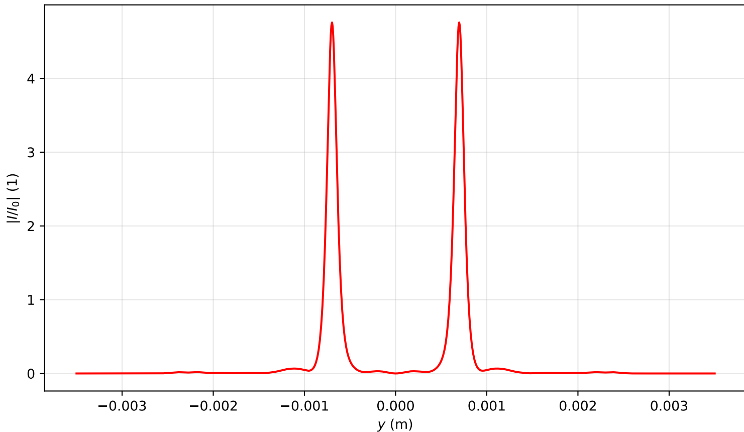
Intensity profile I(x=0, y, z=1.751)/I_0 , P_{in}=15.0P_{cr} , artificial time
