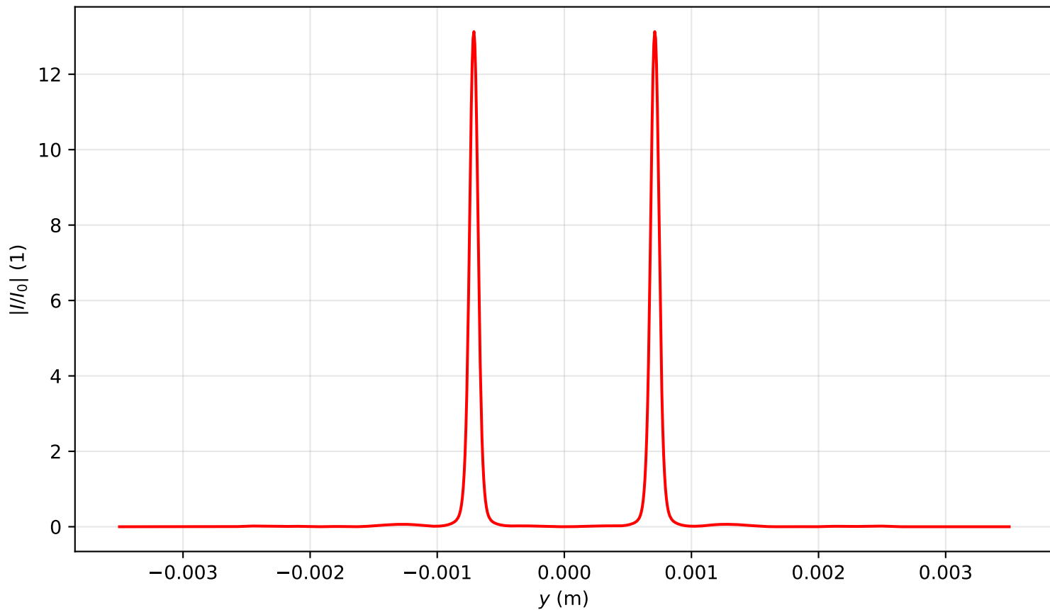
Intensity profile I(x = 0, y, z = 1.831)/I_0 , \text{Pin}=15.0\text{Pcr} , artificial time
