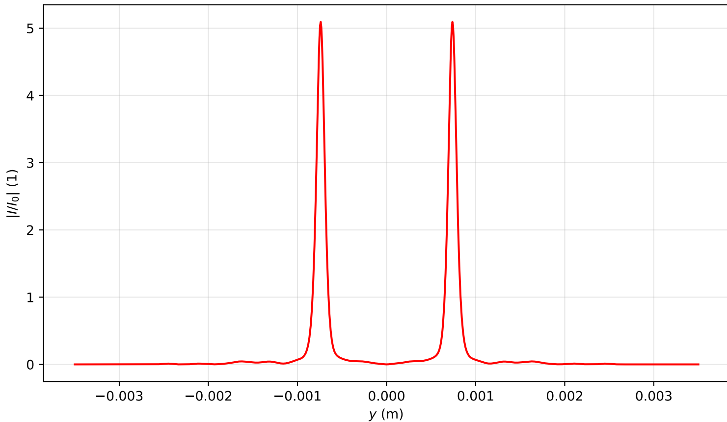
Intensity profile I(x=0, y, z=1.990)/I_0 , P_{in}=15.0\text{Pcr} , artificial time
