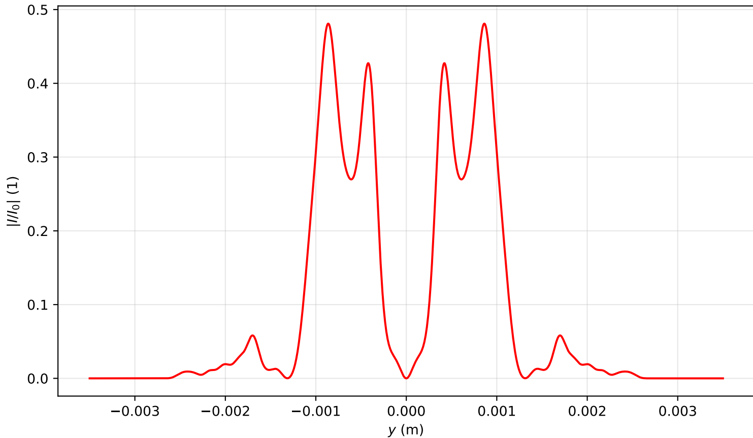
Intensity profile I(x=0, y, z=2.229)/I_0 , P_{in}=15.0P_{cr} , artificial time
