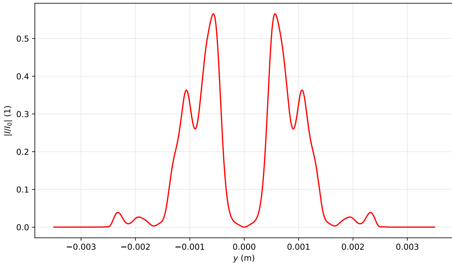
Intensity profile I(x=0, y, z=2.548)/I_0 , P_{in}=15.0P_{cr} , artificial time
