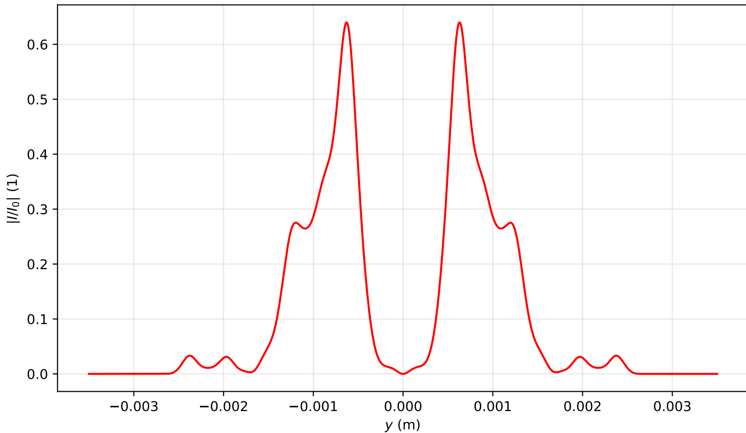
Intensity profile I(x=0, y, z=2.627)/I_0 , P_{in}=15.0\text{Pcr} , artificial time
