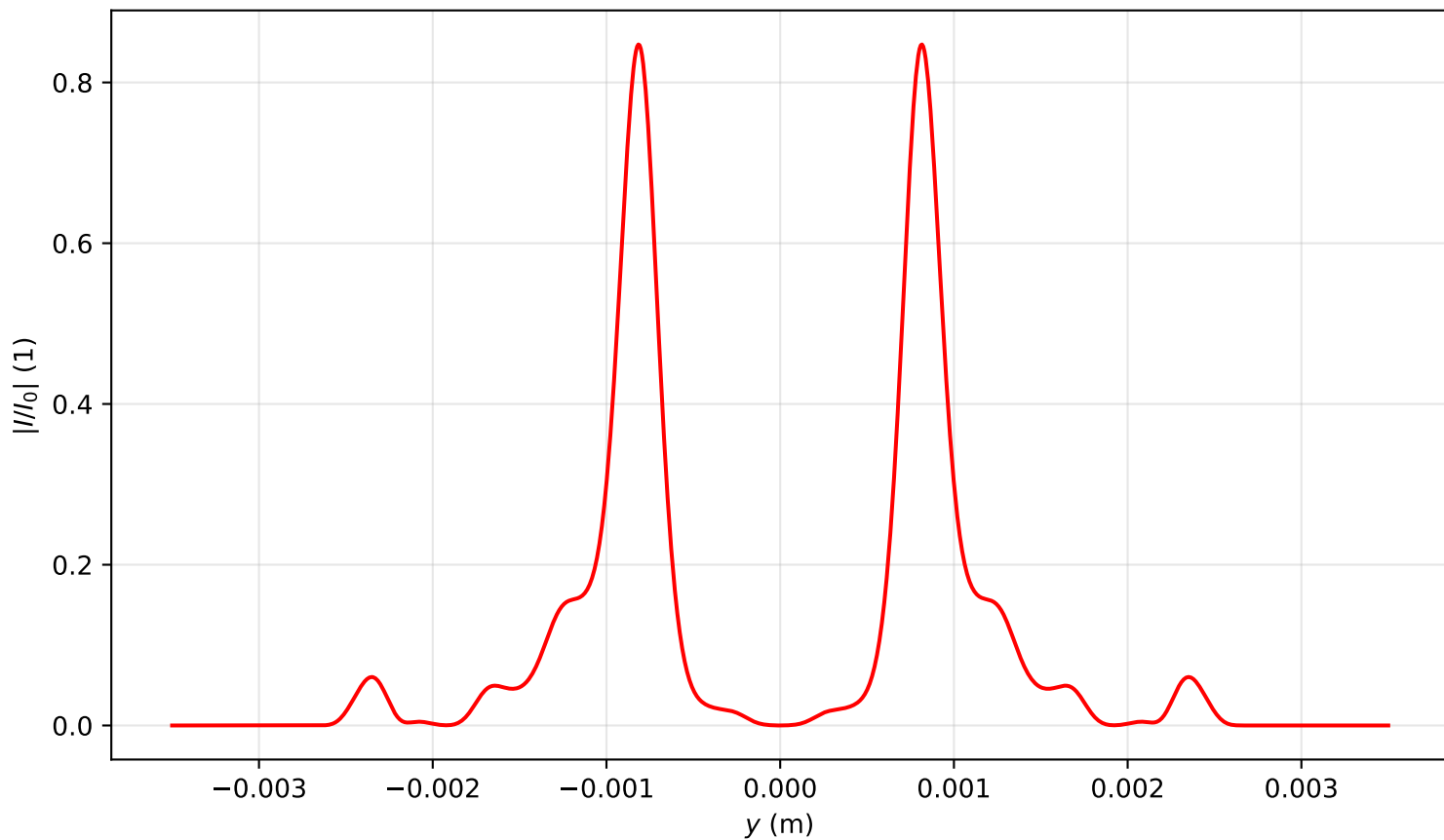
Intensity profile I(x=0, y, z=2.946)/I_0 , P_{in}=15.0P_{cr} , artificial time
