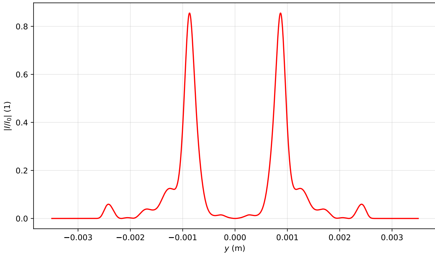
Intensity profile I(x=0, y, z=3.025)/I_0 , P_{in}=15.0P_{cr} , artificial time
