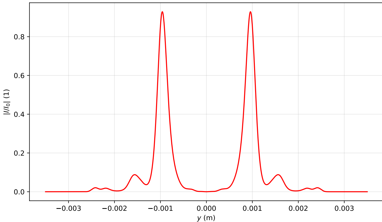
Intensity profile I(x=0, y, z=3.264)/I_0 , P_{in}=15.0\text{Pcr} , artificial time
