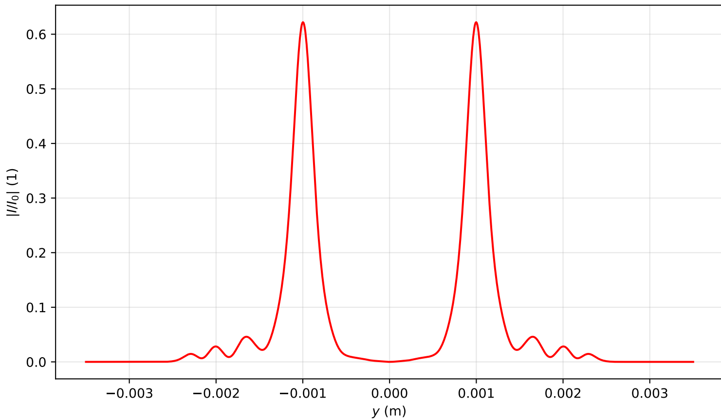
Intensity profile I(x=0, y, z=3.582)/I_0 , P_{in}=15.0\text{Pcr} , artificial time
