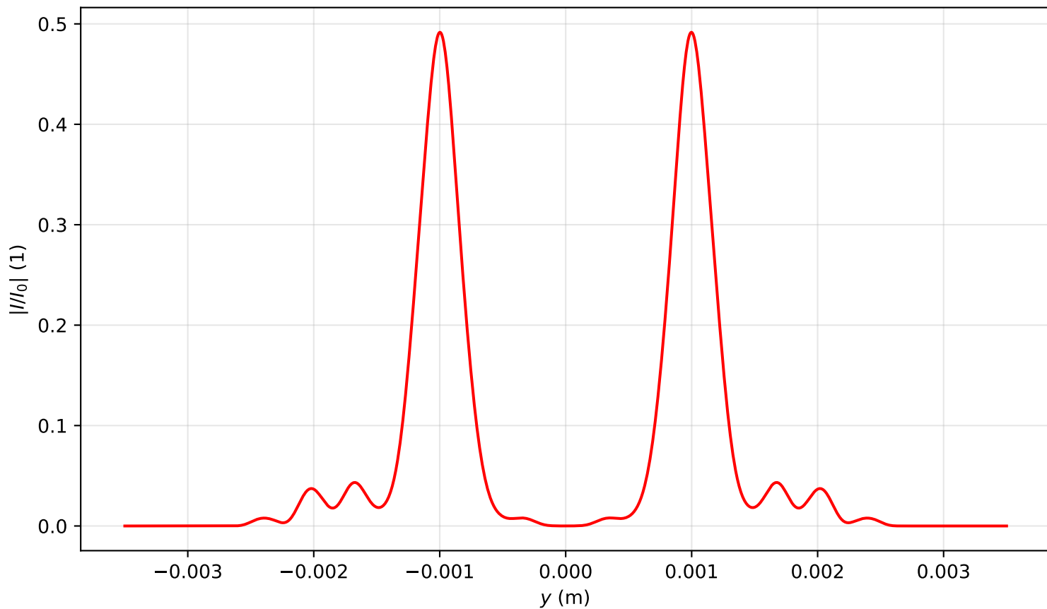
Intensity profile I(x=0, y, z=3.662)/I_0 , P_{in}=15.0P_{cr} , artificial time
