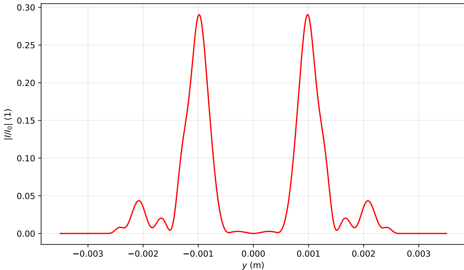
Intensity profile I(x=0, y, z=3.901)/I_0 , P_{in}=15.0\text{Pcr} , artificial time
