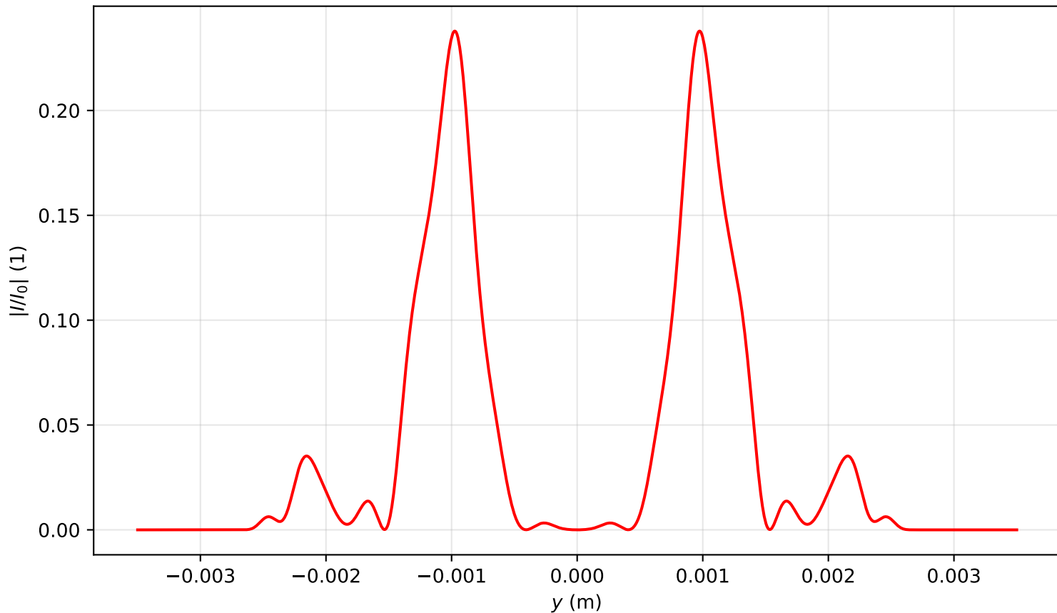
Intensity profile I(x=0, y, z=3.981)/I_0 , P_{in}=15.0P_{cr} , artificial time
