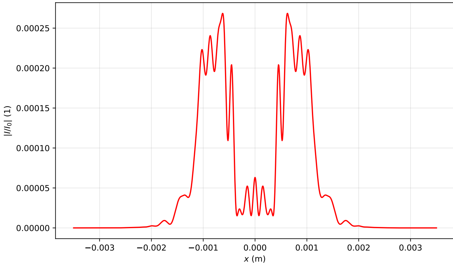
Intensity profile I(x, y = 0, z = 0.557)/I_0 , P_{in}=16.0P_{cr} , artificial time
