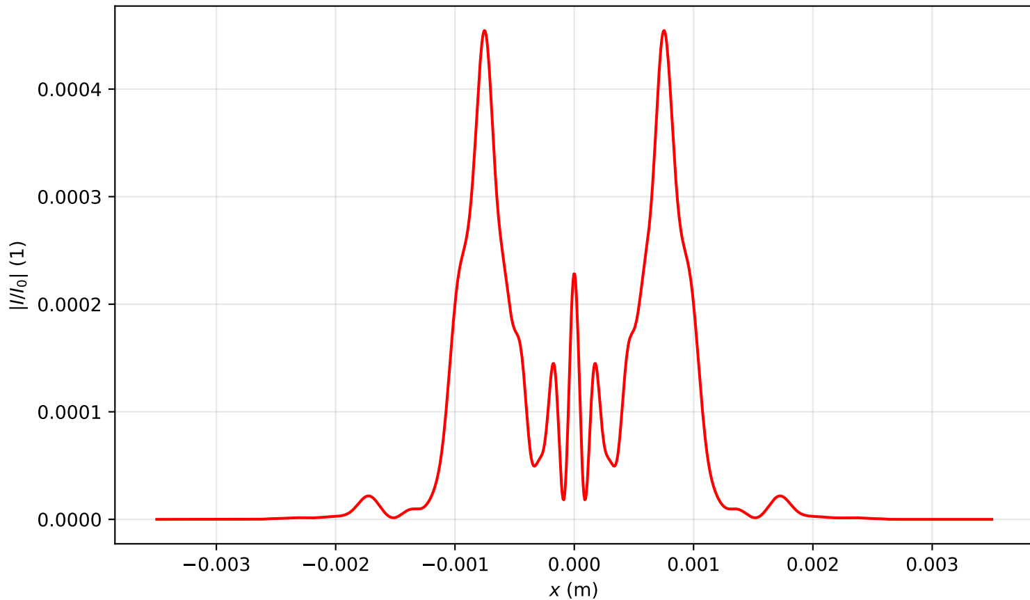
Intensity profile I(x, y = 0, z = 0.716)/I_0 , P_{in}=16.0\text{Pcr} , artificial time
