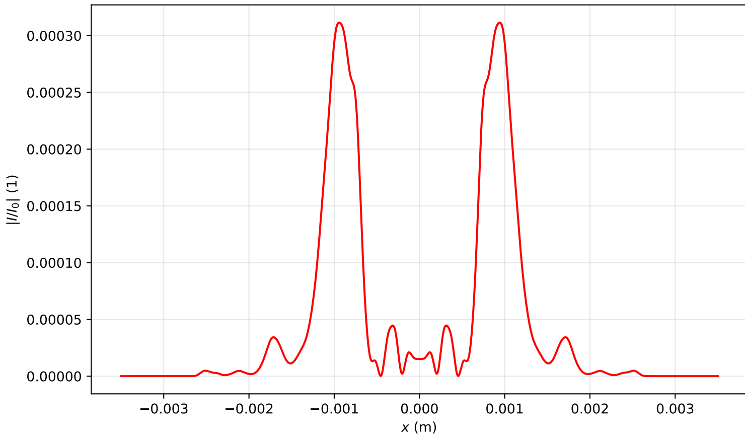
Intensity profile I(x, y = 0, z = 1.513)/I_0 , P_{in}=16.0P_{cr} , artificial time
