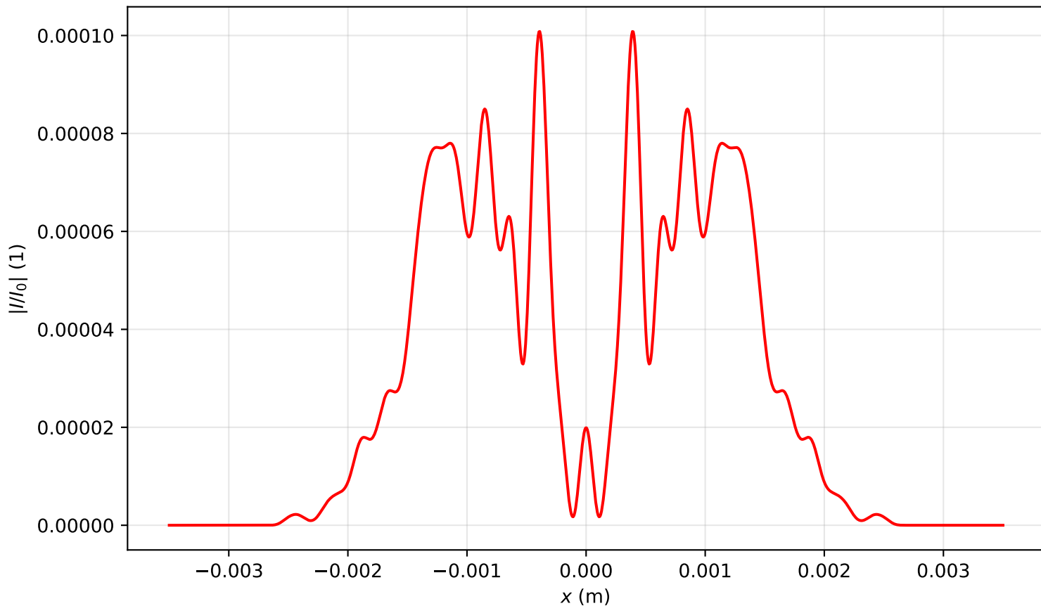
Intensity profile I(x, y = 0, z = 1.831)/I_0 , P_{in}=16.0P_{cr} , artificial time
