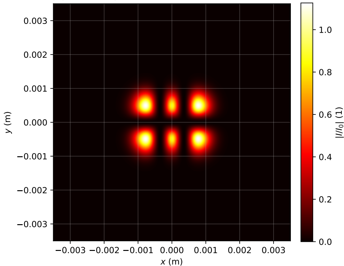
Intensity profile I(x, y, z = 0.080)/I_0 , P_{in}=16.0\text{Pcr} , artificial time
