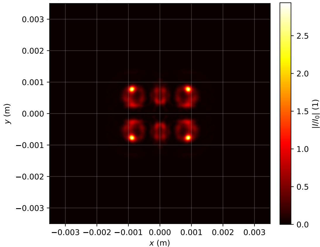
Intensity profile I(x, y, z = 0.637)/I_0 , P_{in}=16.0\text{Pcr} , artificial time
