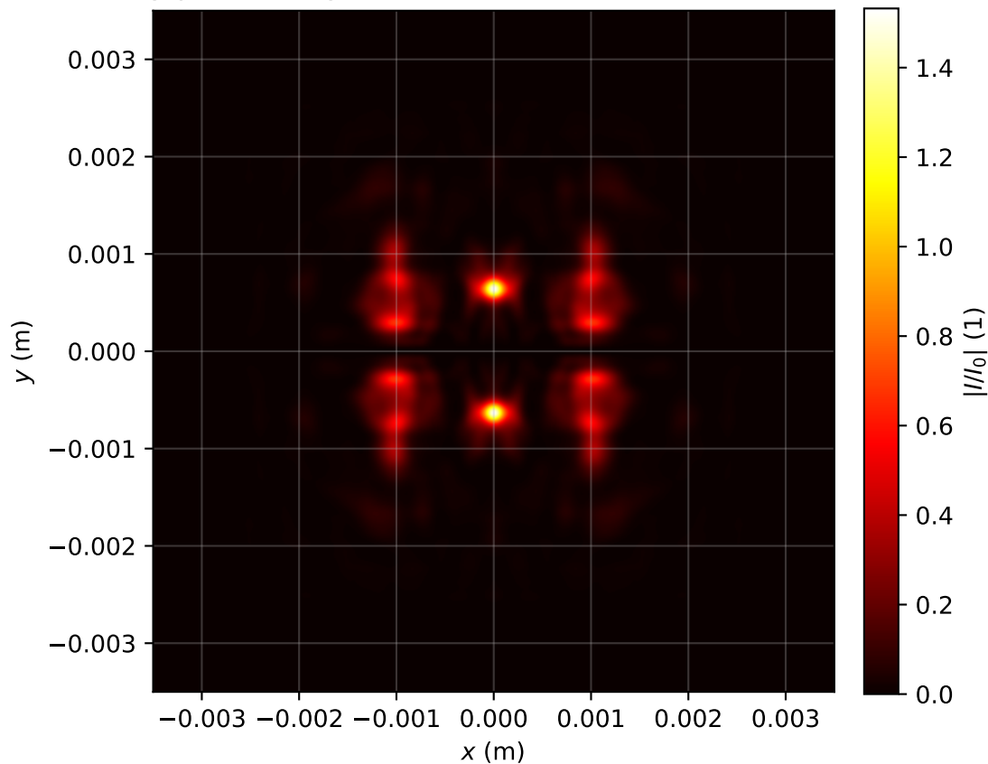
Intensity profile I(x, y, z = 1.513)/I_0 , P_{in}=16.0P_{cr} , artificial time
