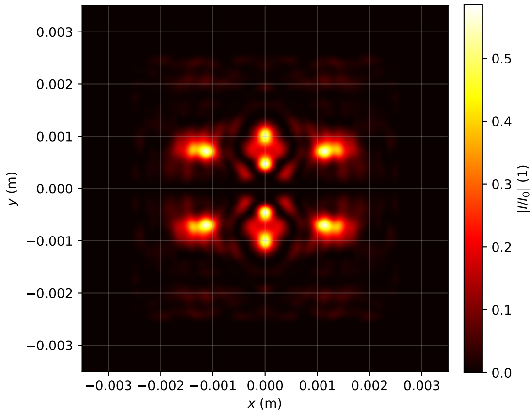
Intensity profile I(x, y, z = 2.229)/I_0 , P_{in}=16.0P_{cr} , artificial time
