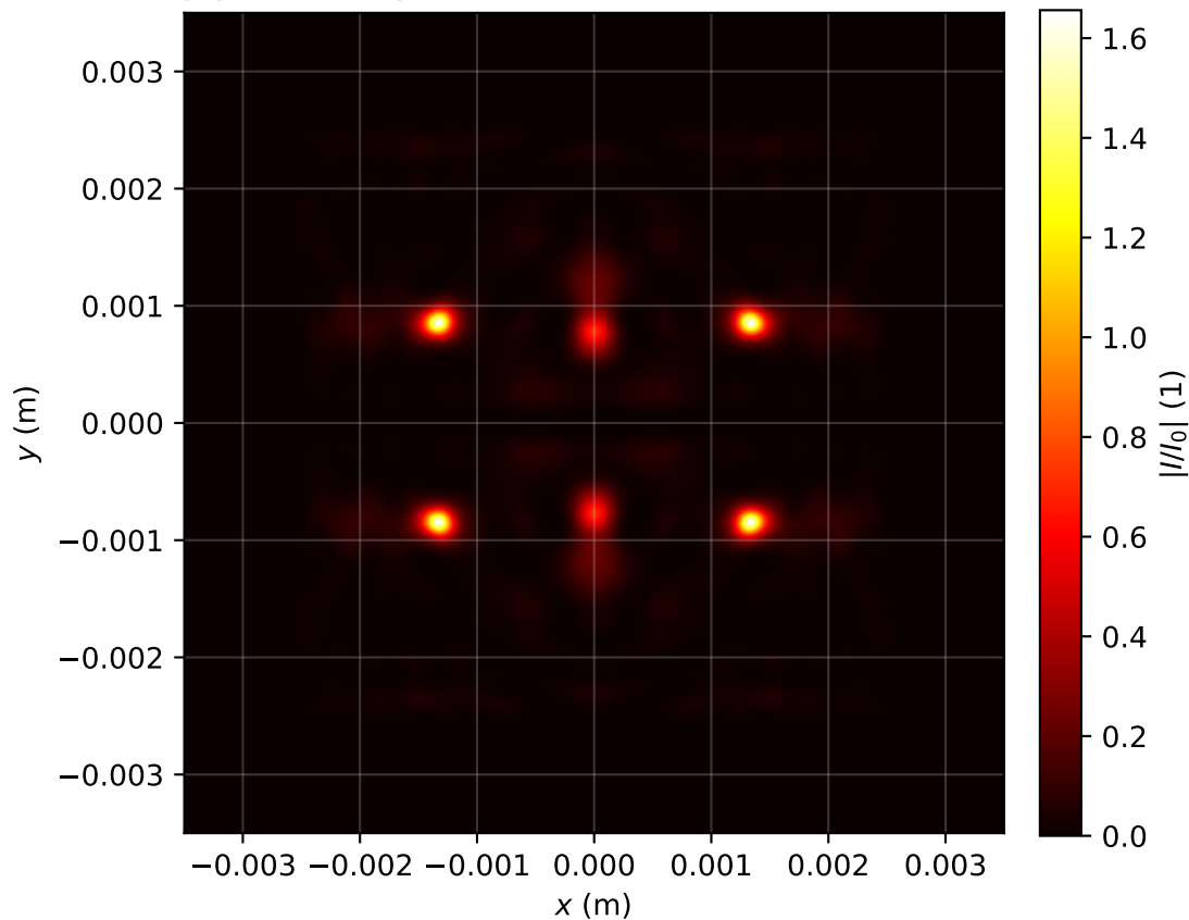
Intensity profile I(x, y, z = 2.707)/I_0 , P_{in}=16.0P_{cr} , artificial time
