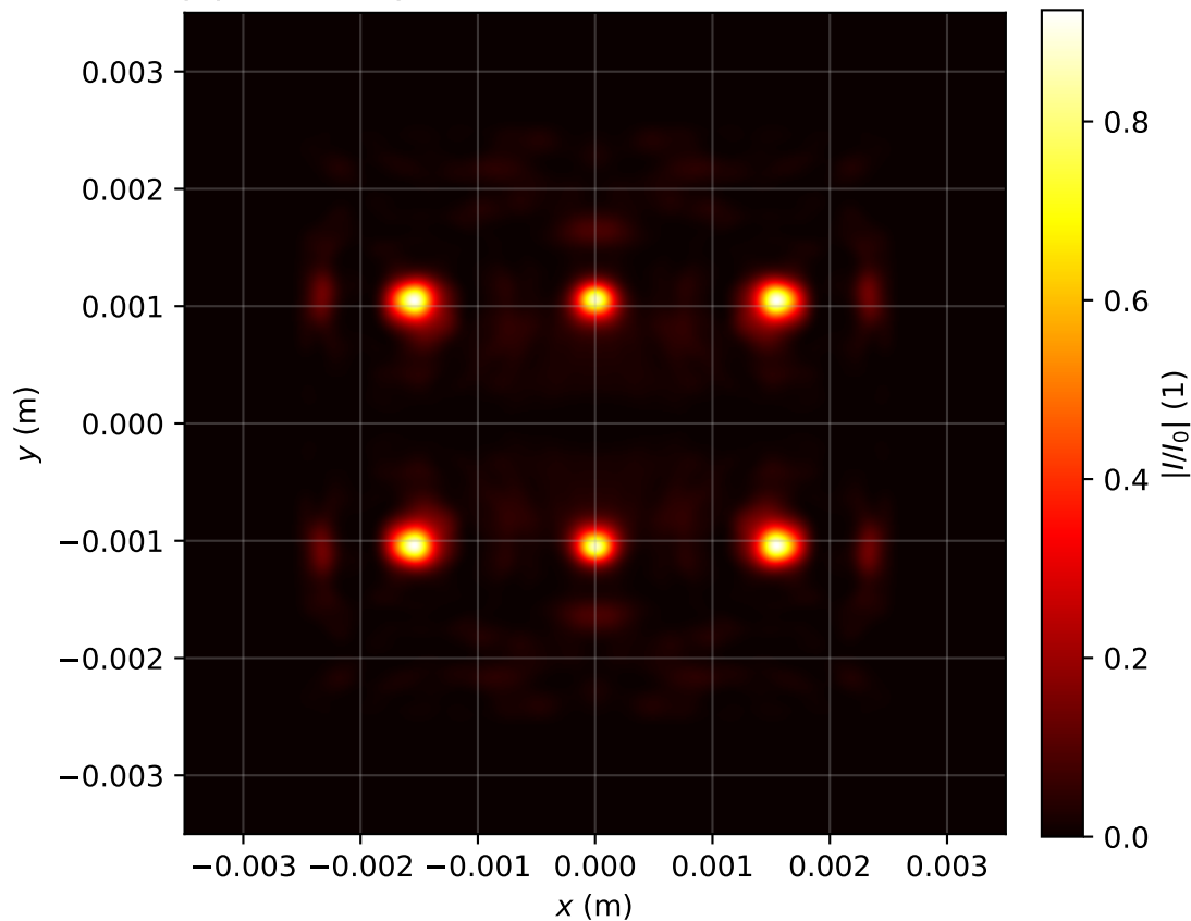
Intensity profile I(x, y, z = 3.344)/I_0 , P_{in}=16.0P_{cr} , artificial time
