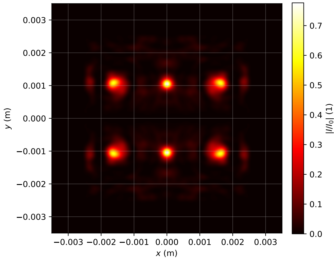
Intensity profile I(x, y, z = 3.423)/I_0 , P_{in}=16.0P_{cr} , artificial time
