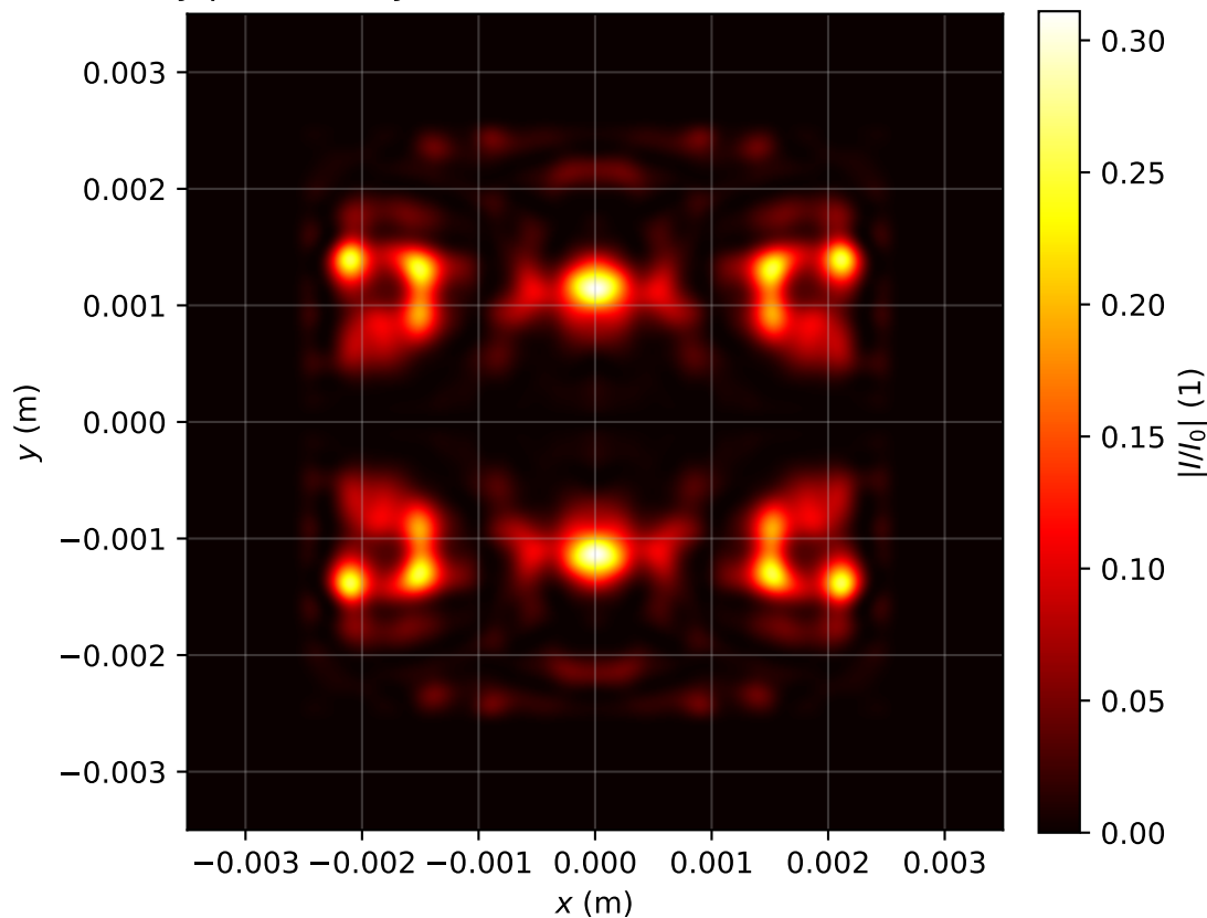
Intensity profile I(x, y, z = 3.981)/I_0 , P_{in}=16.0\text{Pcr} , artificial time
